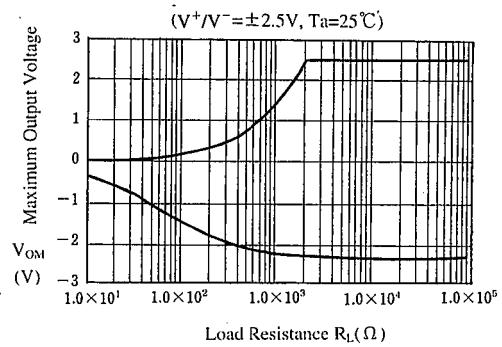
Maximum Output Voltage vs. Load Resistance ( V^+/V^- = \pm 2.5V , T_a = 25^{\circ}C )
