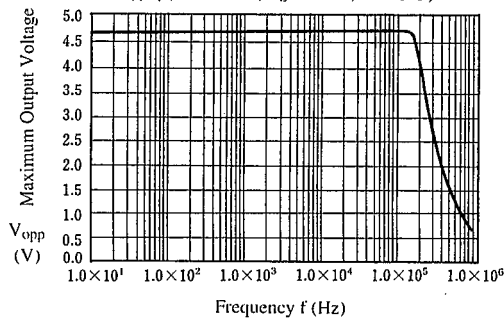
Maximum Output Voltage vs. Frequency ( V^+/V^- = \pm 2.5V , R_L = 2.5k\Omega , T_a = 25^{\circ}C )
