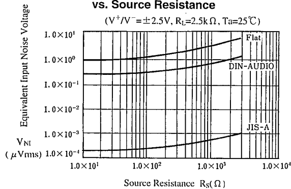
Equivalent Input Noise Voltage vs. Source Resistance ( V^+/V^- = \pm 2.5V , R_L = 2.5k\Omega , T_a = 25^{\circ}C )
