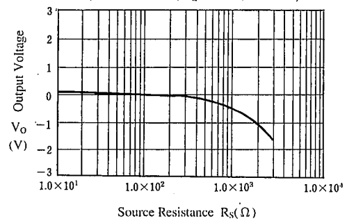
Output Voltage vs. Source Resistance ( V^+/V^- = \pm 2.5V , R_L = 2.5k\Omega , T_a = 25^{\circ}C )
