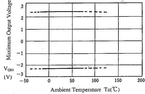
Maximum Output Voltage vs. Temperature ( V^+/V^- = \pm 2.5V , OPEN LOOP, R_L = 2.5k\Omega )
