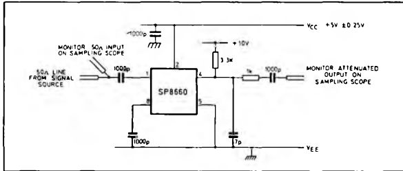
Fig. 3 Test circuit
