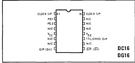
Fig.1 Pin connections
