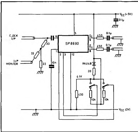
Fig.5 Test circuit for dynamic measurements
