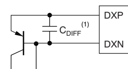
(b) Diode-Connected Transistor
