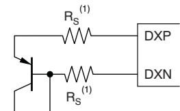
(b) Diode-Connected Transistor
