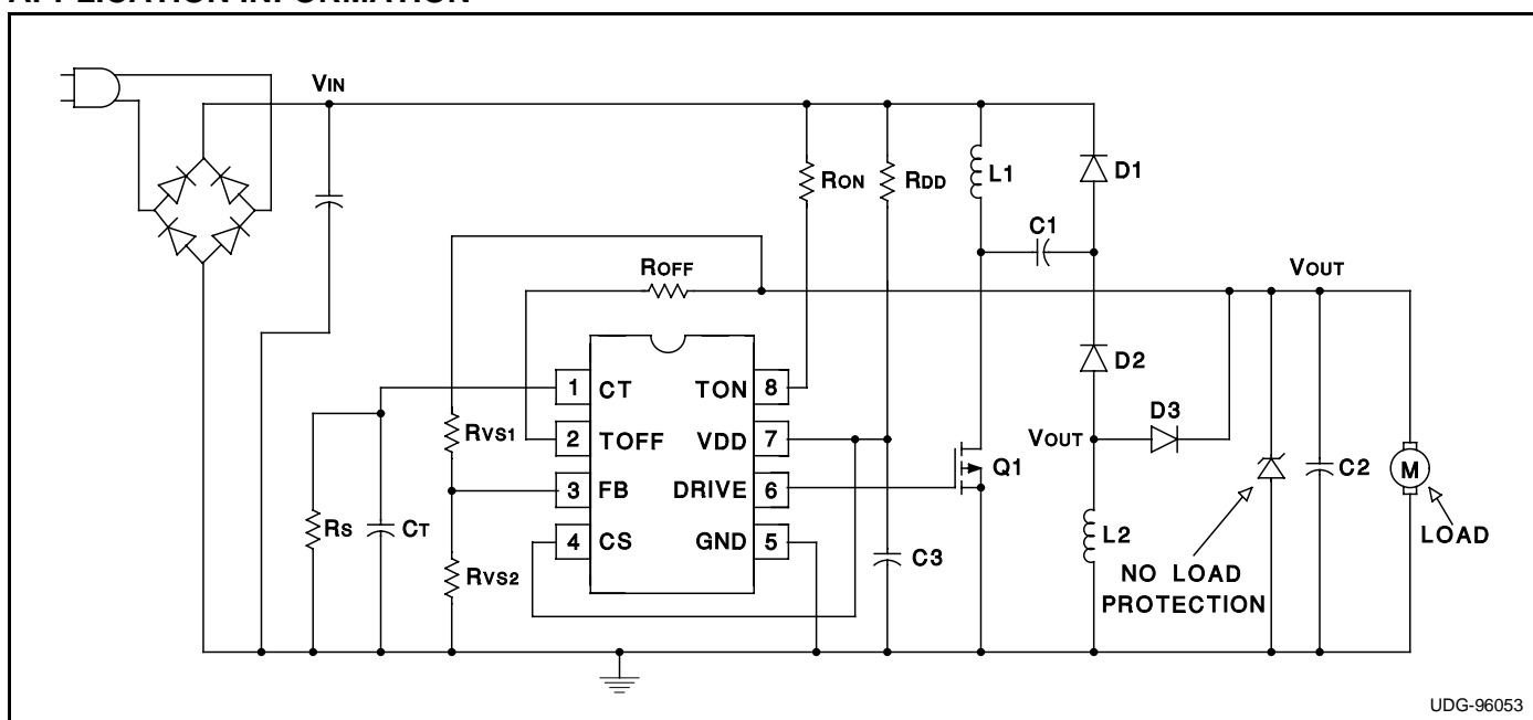
Figure 1. Typical Voltage Mode Application
