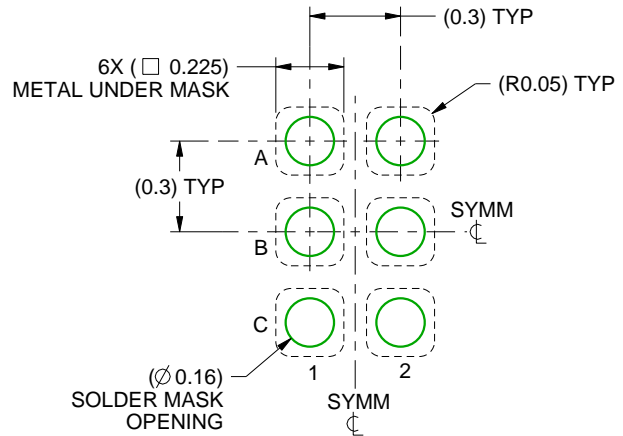
LAND PATTERN EXAMPLE SOLDER MASK DEFINED SCALE:40X
