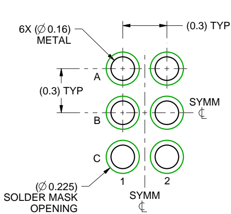
LAND PATTERN EXAMPLE NON-SOLDER MASK DEFINED SCALE:40X
