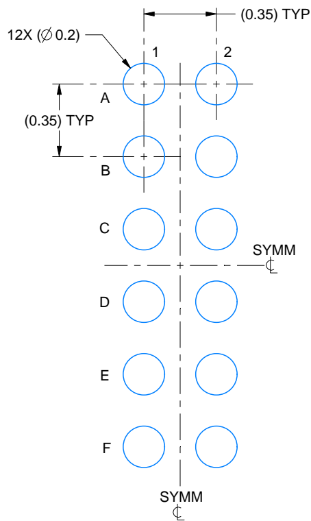
LAND PATTERN EXAMPLE SCALE:40X
