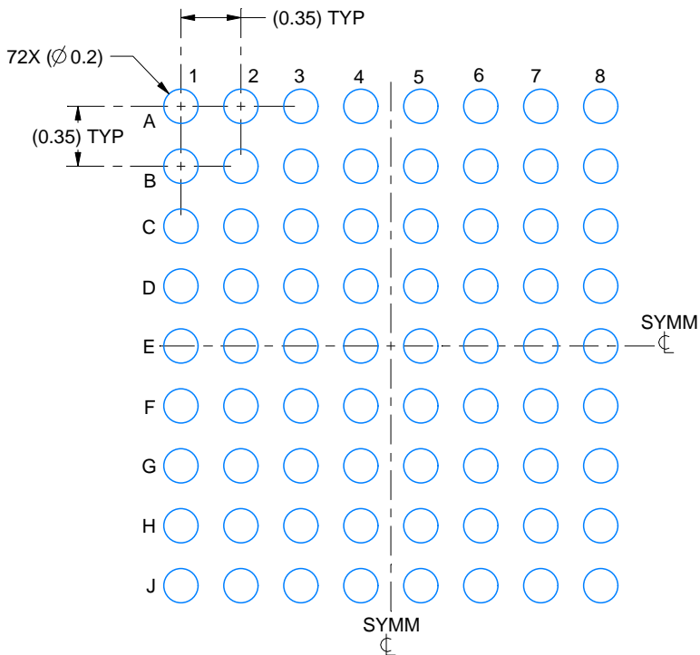
LAND PATTERN EXAMPLE EXPOSED METAL SHOWN SCALE:25X
