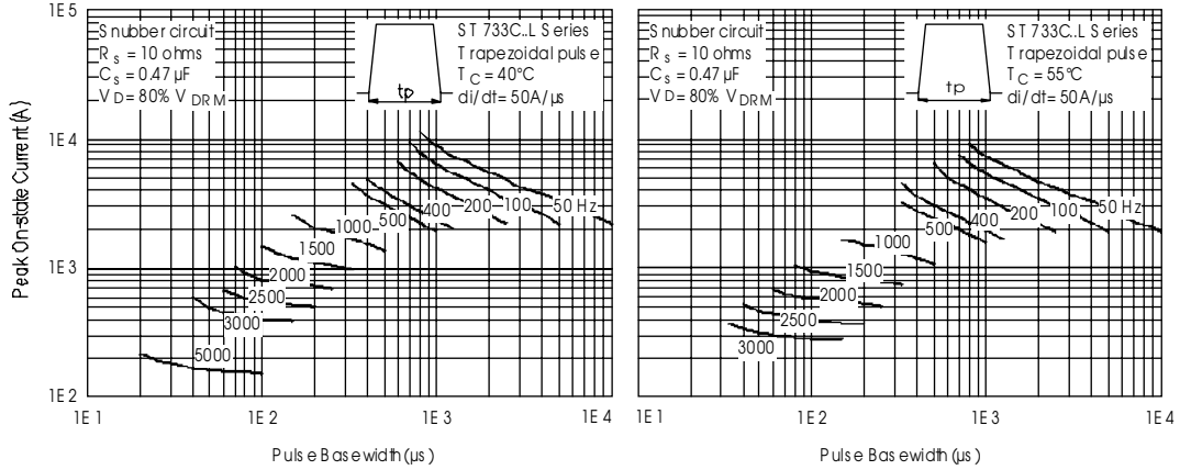
Fig. 14-Frequency Characteristics
