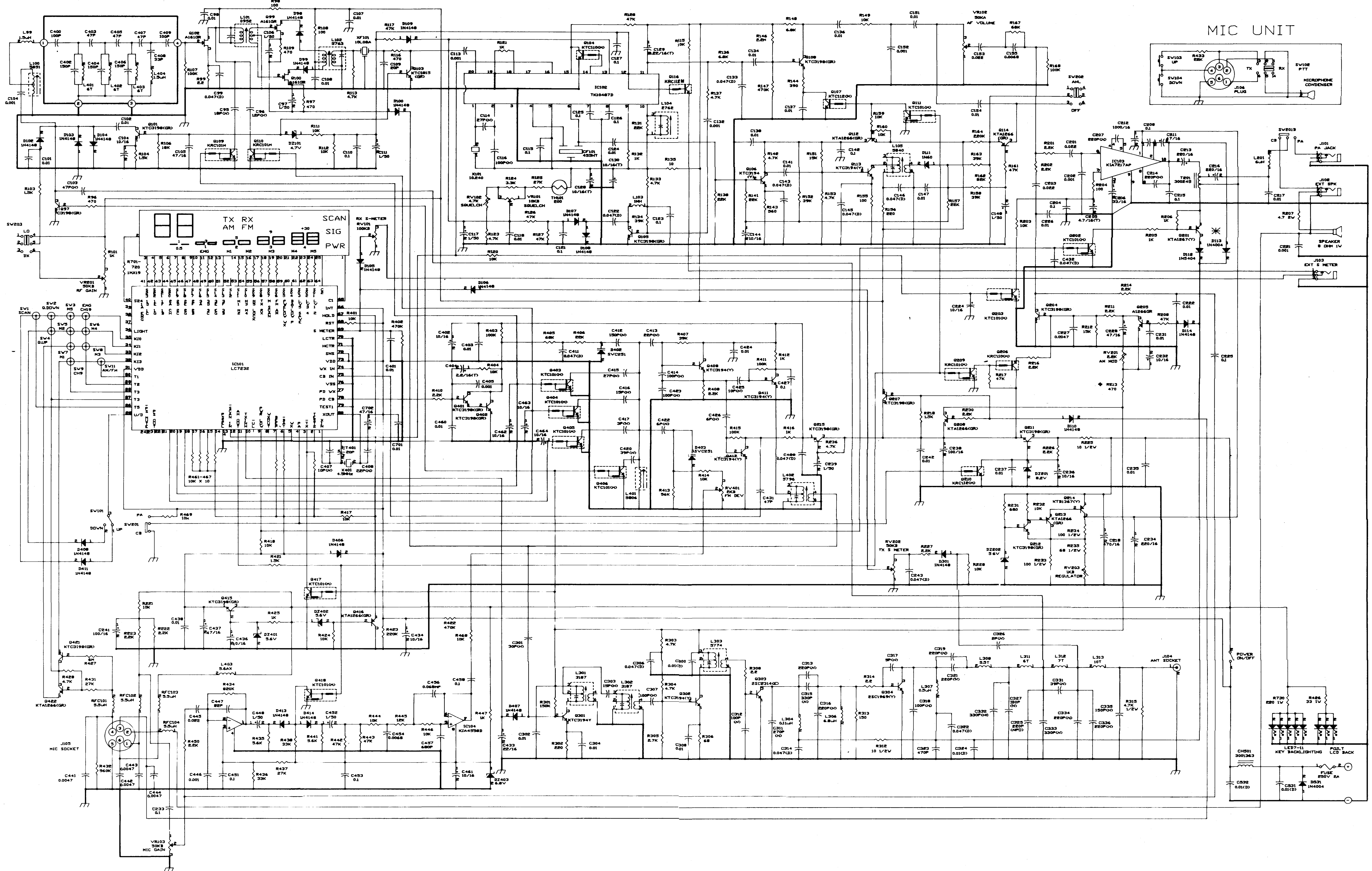
ALAN 48 PLUS SCHEMATIC DIAGRAM
